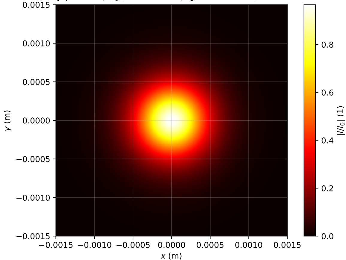
Intensity profile I(x, y, z = 1.911m)/I_0 , P_{in}=0.6P_{cr} , artificial time
